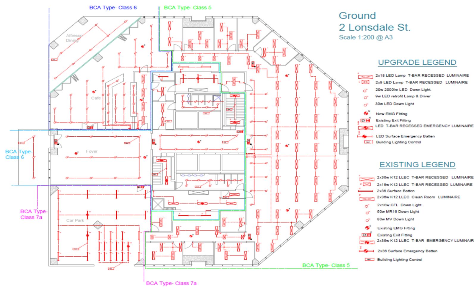
Figure 8: Professionally drafted reflective ceiling plan example – guide only
