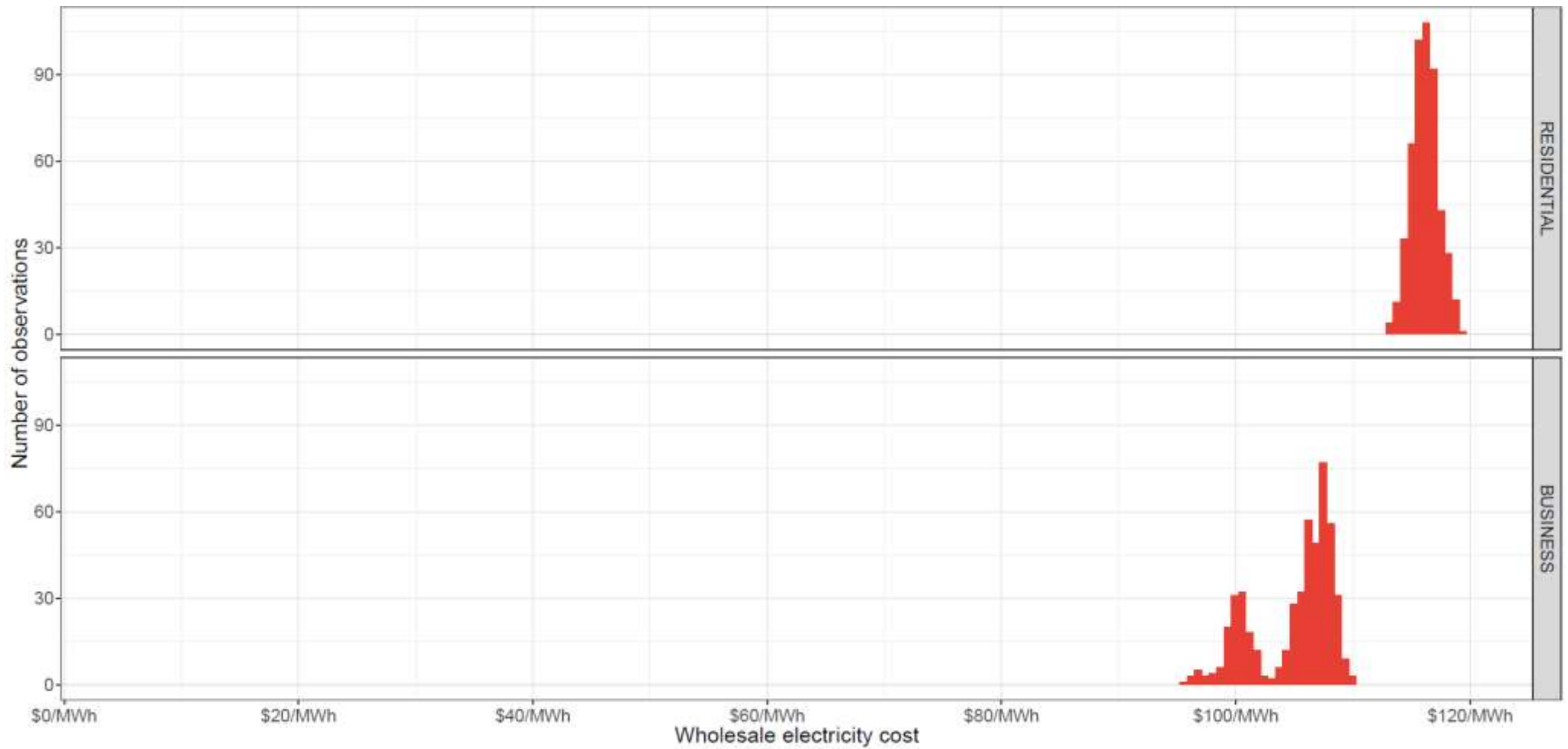
Figure 32: Jemena load wholesale electricity cost distribution
