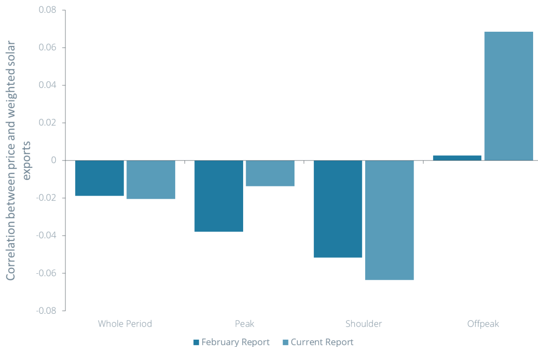
Figure 3: Comparison of correlation between wholesale electricity prices and weighted solar exports
